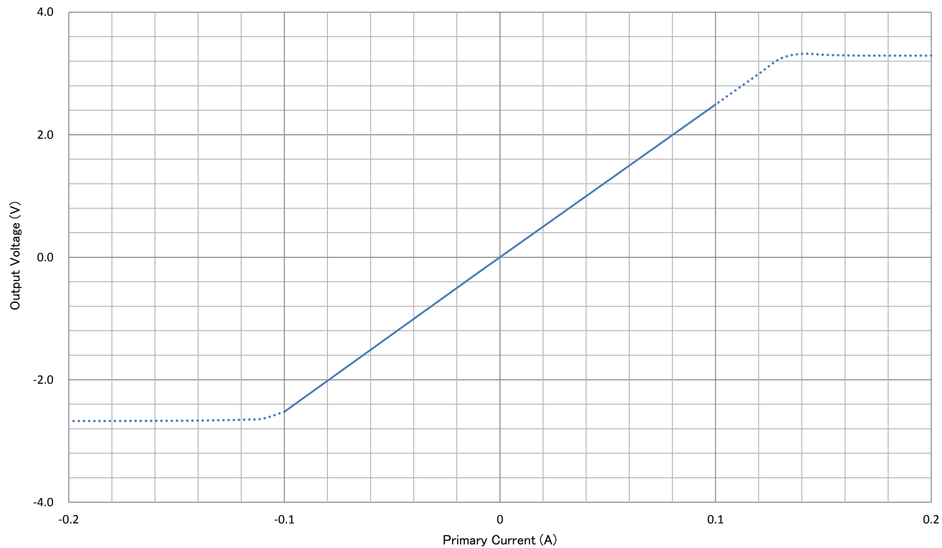
Characteristic of Output Voltage DCZCT-18S
