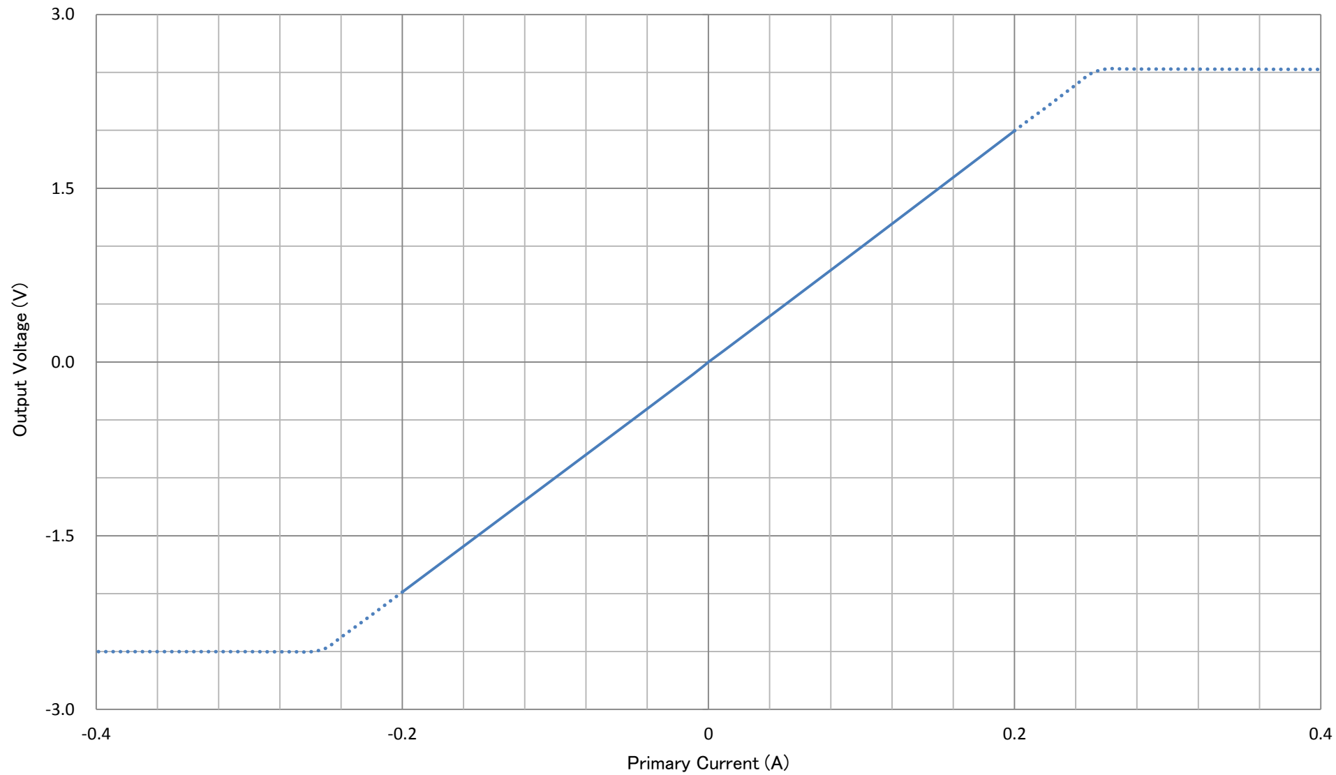
Characteristic of Output Voltage DCZCT-20CDHL
